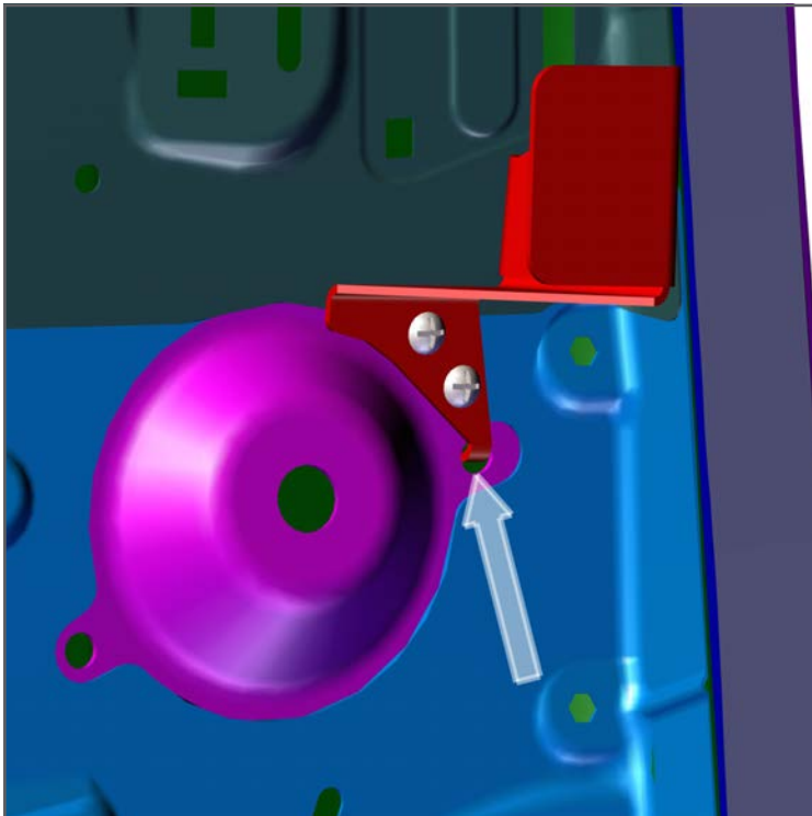
6. Attach the "P/S Armor Upper BKT" by inserting locating tab into place and secure with provide hardware. REPEAT FOR OTHER SIDE.
