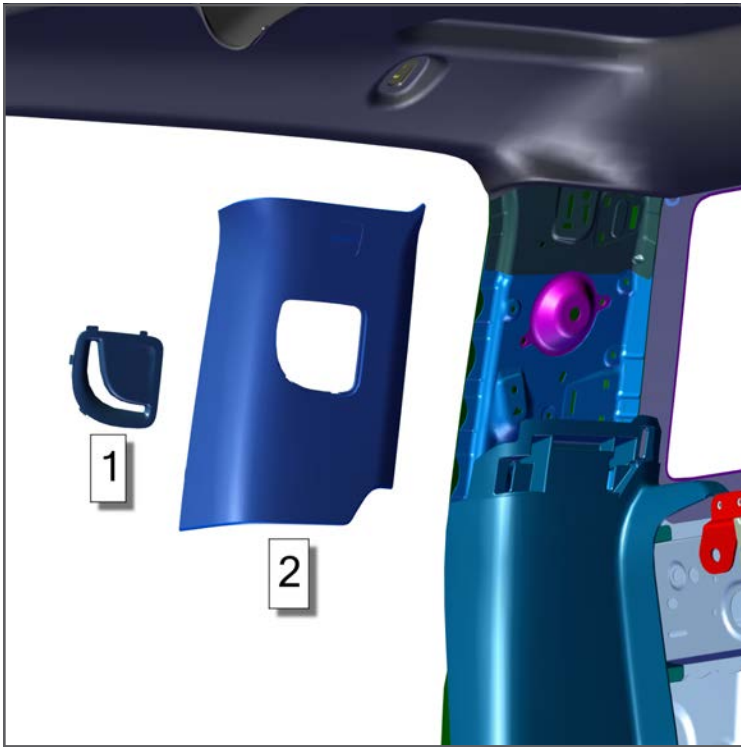
4. Remove "C" pillar upper OEM trim. With a flat trim tool, remove Seatbelt socket guide (1) then the trim (2).
